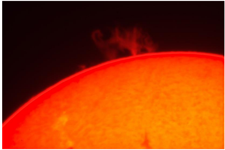
Protuberanzen H-Alpha-Filter
